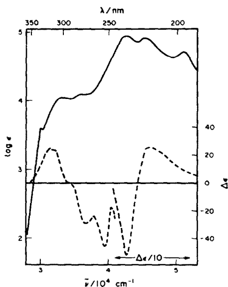
Fig. 2. The absorption (upper curve) and CD spectrum (lower curve) of (R)-(-)-4:4-dimethyldinaphtho [2,1-b,1',2',-d][1,3]dithiepine 2 in ethanol solution.
