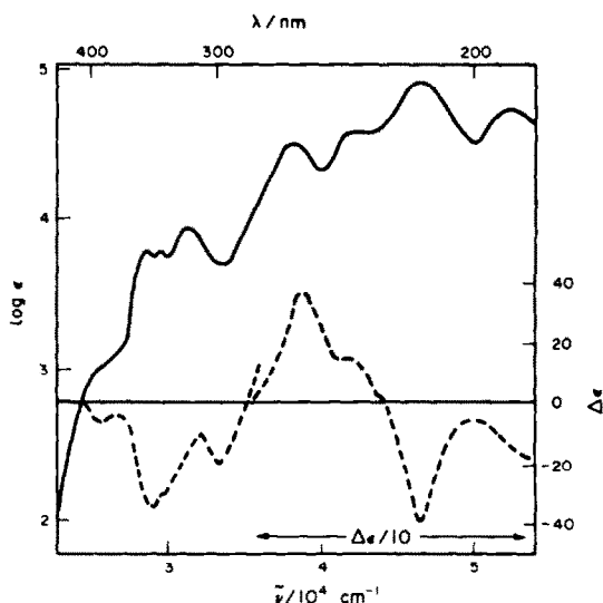
Fig. 1. The absorption (upper curve) and CD spectrum (lower curve) of (S)-(+)-1,1'-binaphthyl-2,2'-disulphide 1 in ethanol solution.
